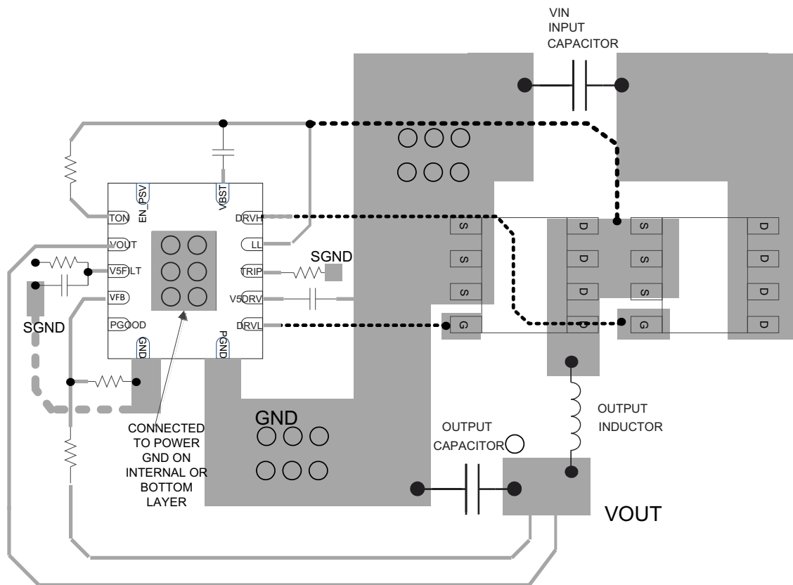
Figure 26. Layout Recommendation
