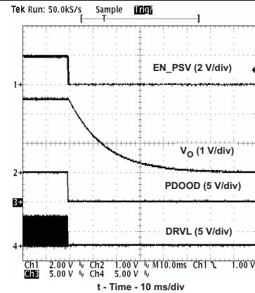
Figure 23. 2.5-V Shutdown Waveforms
