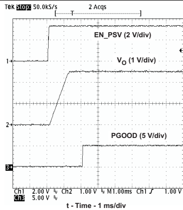
Figure 22. 2.5-V Start-Up Waveforms
