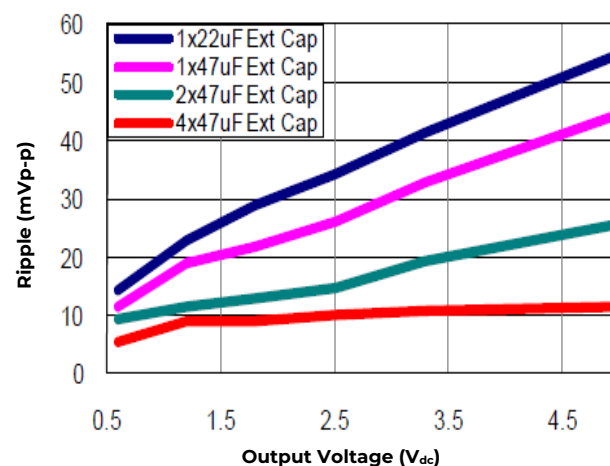
Figure 38. Output ripple voltage for various output voltages with external 1x22 \mu F, 1x47 \mu F, 2x47 \mu F or 4x47 \mu F ceramic capacitors at the output (12A load). Input voltage is 12V.
