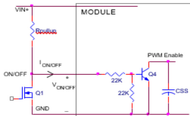
PVX012 NEGATIVE LOGIC FIGURE
