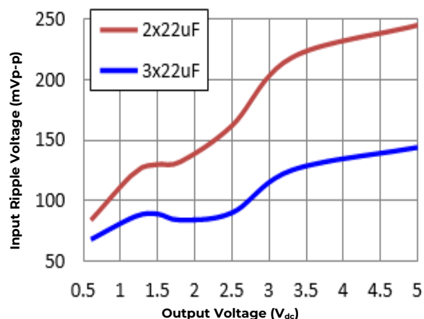
Figure 37. Input ripple voltage for various output voltages with 2x22 \mu F or 3x22 \mu F ceramic capacitors at the input (12A load). Input voltage is 12V.
