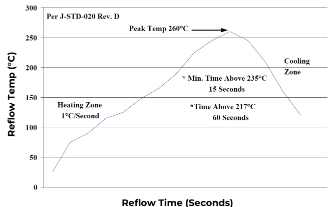
Figure 48. Recommended linear reflow profile using Sn/Ag/Cu solder.
