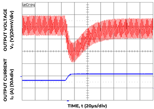
Figure 22. Transient Response to Dynamic Load Change from 50% to 100% at 12V in , C out =1x47μF+1x330μF, C Tune =3300pF, R Tune =270ohms
