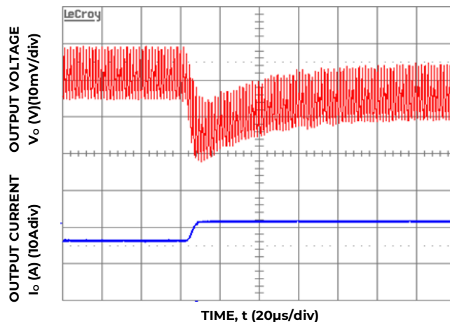
Figure 10. Transient Response to Dynamic Load Change from 50% to 100% at 12V in , C out -1x47μF+3x330μF, C Tune -10nF, R Tune -220ohms
