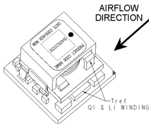
Figure 47. Preferred airflow direction and location of hot-spot of the module ( T_{ref} ).
