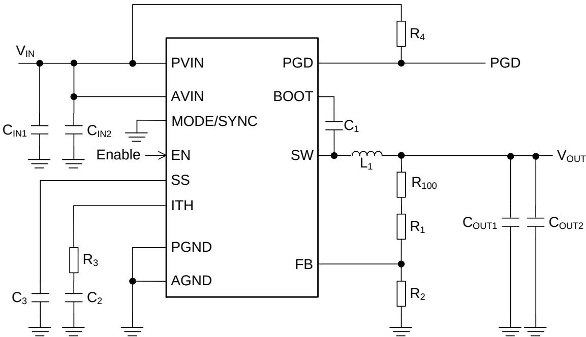
Figure 34. Typical Application
