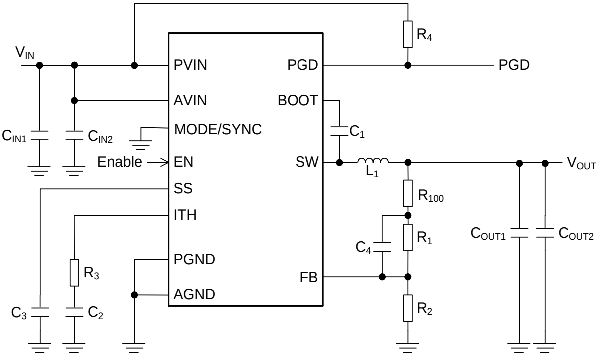
Figure 51. Reference Circuit 3
