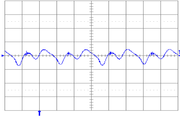
Fig. 1.2V.7: Output voltage ripple (20 mV/div.) at full rated load current into a resistive load with C_o = 10\ \mu\text{F} tantalum + 1 \mu\text{F} ceramic and V_{in} = 48\ \text{V} . Time scale: 1 \mu\text{s}/\text{div} .
