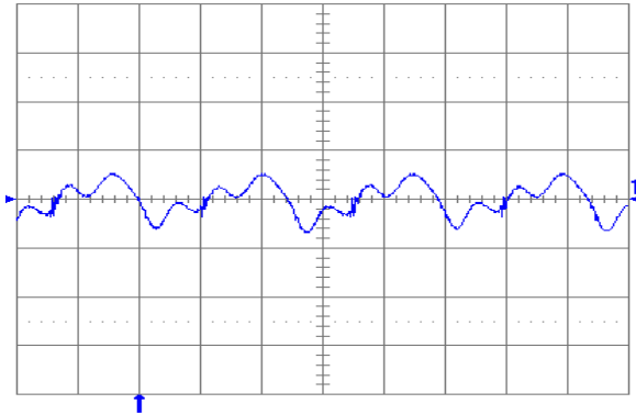
Fig. 1.8V.7: Output voltage ripple (20mV/div.) at full rated load current into a resistive load with C_o = 10\ \mu\text{F} tantalum + 1 \mu\text{F} ceramic and V_{in} = 48\ \text{V} . Time scale: 1 \mu\text{s}/\text{div} .
