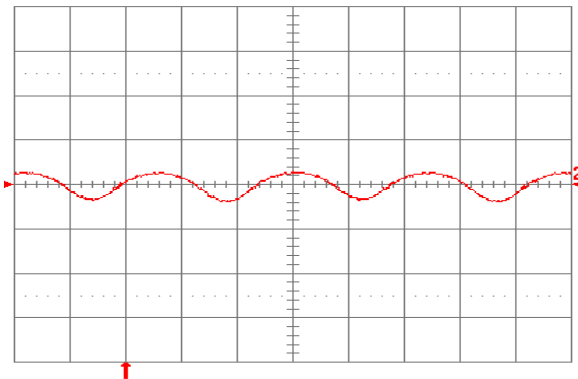
Fig. 1.5V.9: Input reflected ripple current, i_c (100 A/div.), measured at input terminals at full rated load current and V_{in} = 48\ \text{V} . Refer to Fig. 1.5V.8 for test setup. Time scale: 1 \mu\text{s}/\text{div} .
