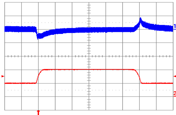
Fig. 3.3V.5: Output voltage response to load current step-change (5A – 10A – 5A ) at V_{in} = 48 V. Top trace: output voltage (100 mV/div.). Bottom trace: load current (5A/div.). Current slew rate: 0.1 A/ \mu s. C_o = 1 \mu F ceramic. Time scale: 0.2 ms/div.
