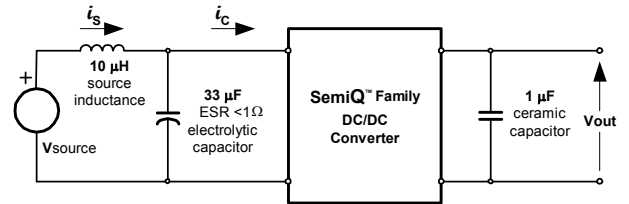
Fig. 1.2V.8: Test setup for measuring input reflected ripple currents, i_c and i_s
