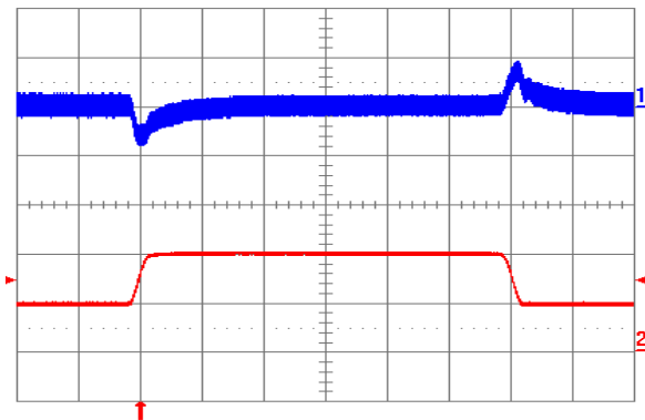
Fig. 1.2V.5: Output voltage response to load current step-change (5A – 10A – 5A) at V_{in} = 48 V. Top trace: output voltage (100 mV/div.). Bottom trace: load current (5 A/div.). Current slew rate: 0.1A/ \mu s. C_o = 1 \mu F ceramic. Time scale: 0.2 ms/div.
