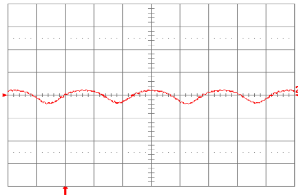
Fig. 1.2V.9: Input reflected ripple current, i_c (100mA/div.), measured at input terminals at full rated load current and V_{in} = 48\ \text{V} . Refer to Fig. 1.2V.8 for test setup. Time scale: 1 \mu\text{s}/\text{div} .
