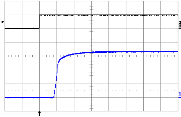
Fig. 3.3V.3: Turn-on transient at full rated load current (resistive) with no output capacitor at V_{in} = 48 V, triggered via ON/OFF pin. Top trace: ON/OFF signal (5V/div.). Bottom trace: output voltage (1 V/div.). Time scale: 2 ms/div.
