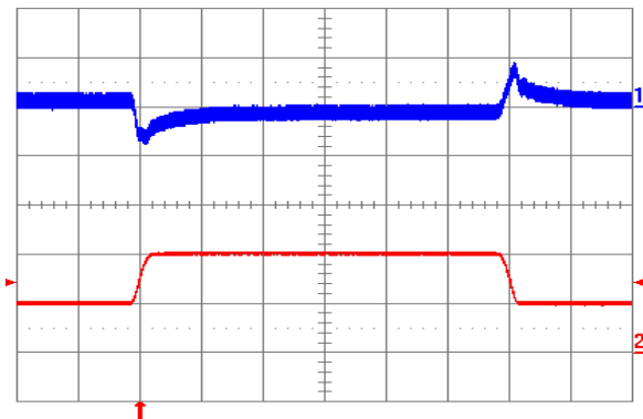
Fig. 1.8V.5: Output voltage response to load current step-change (5A – 10A – 5A) at V_{in} = 48 V. Top trace: output voltage (100 mV/div.). Bottom trace: load current (5 A/div.). Current slew rate: 0.1A/ \mu s. C_o = 1 \mu F ceramic. Time scale: 0.2 ms/div.
