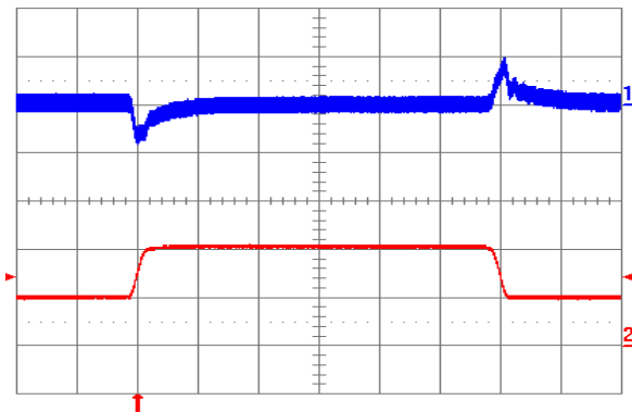
Fig. 1.5V.5: Output voltage response to load current step-change (5A – 10A – 5A) at V_{in} = 48 V. Top trace: output voltage (100 mV/div.). Bottom trace: load current (5 A/div.). Current slew rate: 0.1 A/ \mu s. C_o = 1 \mu F ceramic. Time scale: 0.2 ms/div.
