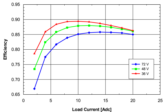
Fig. 1.8V.2: Efficiency vs. load current and input voltage for SQM48T/S20018 converter mounted vertically with air flowing from pin 3 to pin 1 at a rate of 300 LFM (1.5 m/s) and T_a = 25^\circ\text{C} .
