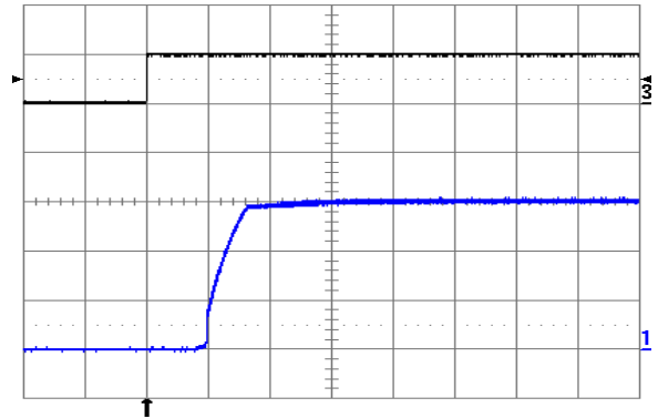
Fig. 1.5V.4: Turn-on transient at full rated load current (resistive) plus 10,000 \mu F at V_{in} = 48 V, triggered via ON/OFF pin. Top trace: ON/OFF signal (5 V/div.). Bottom trace: output voltage (0.5 V/div.). Time scale: 2 ms/div.
