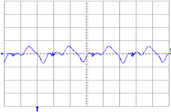
Fig. 1.5V.7: Output voltage ripple (20 mV/div.) at full rated load current into a resistive load with C_o = 10\ \mu\text{F} tantalum + 1 \mu\text{F} ceramic and V_{in} = 48\ \text{V} . Time scale: 1 \mu\text{s}/\text{div} .
