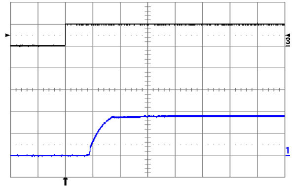
Fig. 1.8V.4: Turn-on transient at full rated load current (resistive) plus 10,000 \mu F at V_{in} = 48 V, triggered via ON/OFF pin. Top trace: ON/OFF signal (5 V/div.). Bottom trace: output voltage (1 V/div.). Time scale: 2 ms/div.
