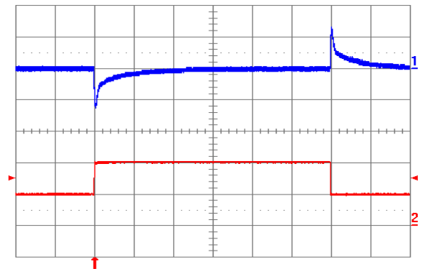
Fig. 3.3V.6: Output voltage response to load current step-change (5A – 10A – 5A) at V_{in} = 48 V. Top trace: output voltage (100 mV/div.). Bottom trace: load current (5 A/div.). Current slew rate: 5 A/ \mu s. C_o = 450 \mu F tantalum + 1 \mu F ceramic. Time scale: 0.2 ms/div.
