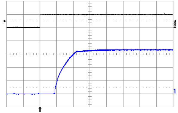
Fig. 3.3V.4: Turn-on transient at full rated load current (resistive) plus 10,000 \mu F at V_{in} = 48 V, triggered via ON/OFF pin. Top trace: ON/OFF signal (5 V/div.). Bottom trace: output voltage (1 V/div.). Time scale: 2 ms/div.
