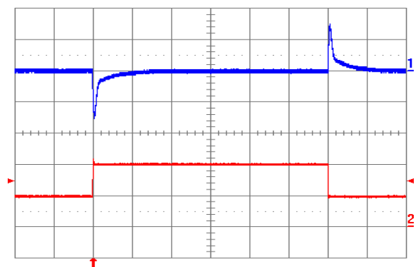
Fig. 1.5V.6: Output voltage response to load current step-change (5A – 10A – 5A) at V_{in} = 48 V. Top trace: output voltage (100 mV/div.). Bottom trace: load current (5 A/div.). Current slew rate: 5 A/ \mu s. C_o = 450 \mu F tantalum + 1 \mu F ceramic. Time scale: 0.2 ms/div.
