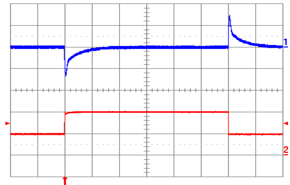
Fig. 1.8V.6: Output voltage response to load current step-change (5A – 10A – 5A) at V_{in} = 48 V. Top trace: output voltage (100 mV/div.). Bottom trace: load current (5 A/div.). Current slew rate: 5 A/ \mu s. C_o = 450 \mu F tantalum + 1 \mu F ceramic. Time scale: 0.2 ms/div.
