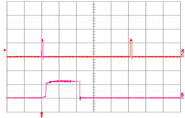
Fig. 3.3V.12: Load current (top trace, 20 A/div., 20ms/div.) into a 10 mΩ short circuit during restart, at V_{in} = 48 V. Bottom trace (20 A/div., 1ms/div.) is an expansion of the on-time portion of the top trace.
