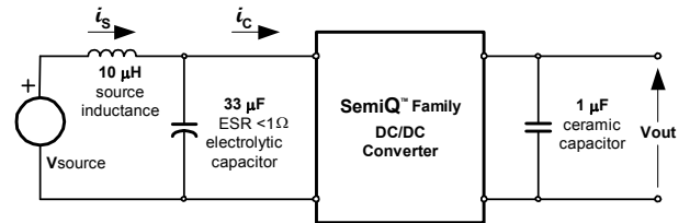
Fig. 3.3V.8: Test setup for measuring input reflected ripple currents, i_c and i_s .
