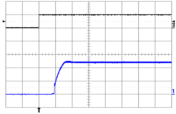
Fig. 1.2V.4: Turn-on transient at full rated load current (resistive) plus 10,000 \mu F at V_{in} = 48 V, triggered via ON/OFF pin. Top trace: ON/OFF signal (5 V/div.). Bottom trace: output voltage (0.5 V/div.). Time scale: 2 ms/div.
