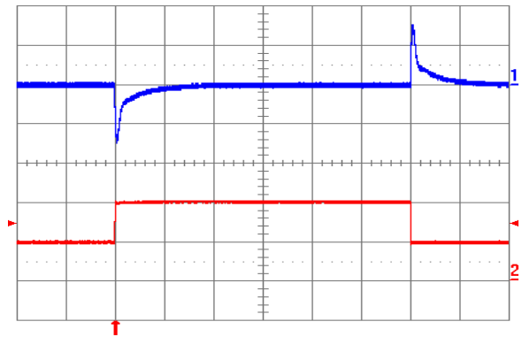
Fig. 1.2V.6: Output voltage response to load current step-change (5A – 10A – 5A) at V_{in} = 48 V. Top trace: output voltage (100 mV/div.). Bottom trace: load current (5 A/div.). Current slew rate: 5 A/ \mu s. C_o = 450 \mu F tantalum + 1 \mu F ceramic. Time scale: 0.2 ms/div.
