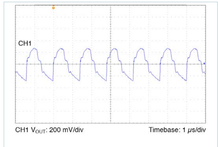
Figure 18 — Output voltage ripple, V_{IN} = 28\text{V} , V_{OUT} = 15.0\text{V} , C_{OUT\_EXT} = 680\mu\text{F} , R_{LOAD} = 0.701\Omega
