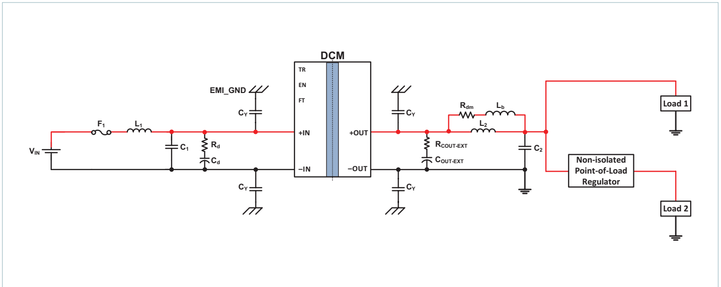
Typical application 1: single DCM3623x50M17C2y7z to a non-isolated regulator and direct to load
