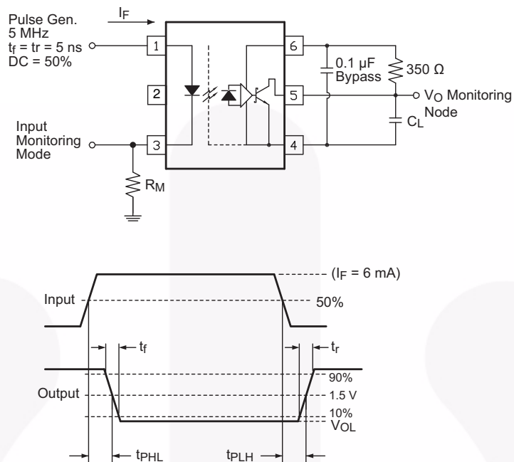
Figure 16. Test Circuit for Propagation Delay, Rise Time, and Fall Time
