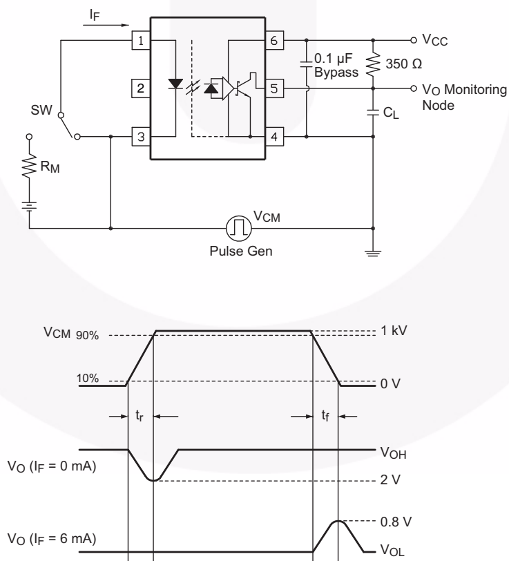
Figure 17. Test Circuit for Instantaneous Common-Mode Rejection Voltage
