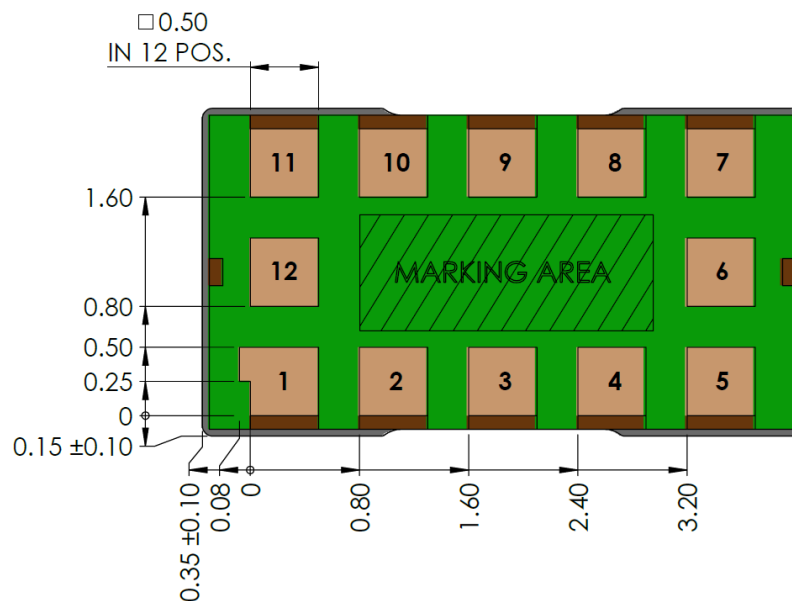
Figure 18. Outline drawing 3/5
