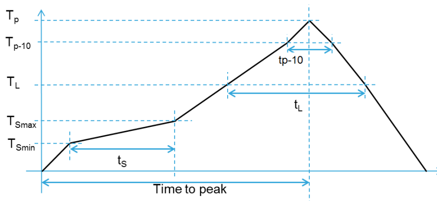
Figure 24. Solder profile
