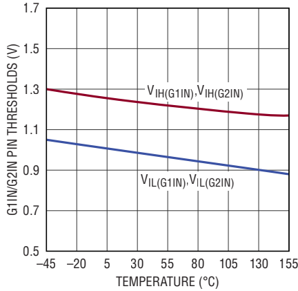
G1IN/G2IN Pin Thresholds vs Temperature
