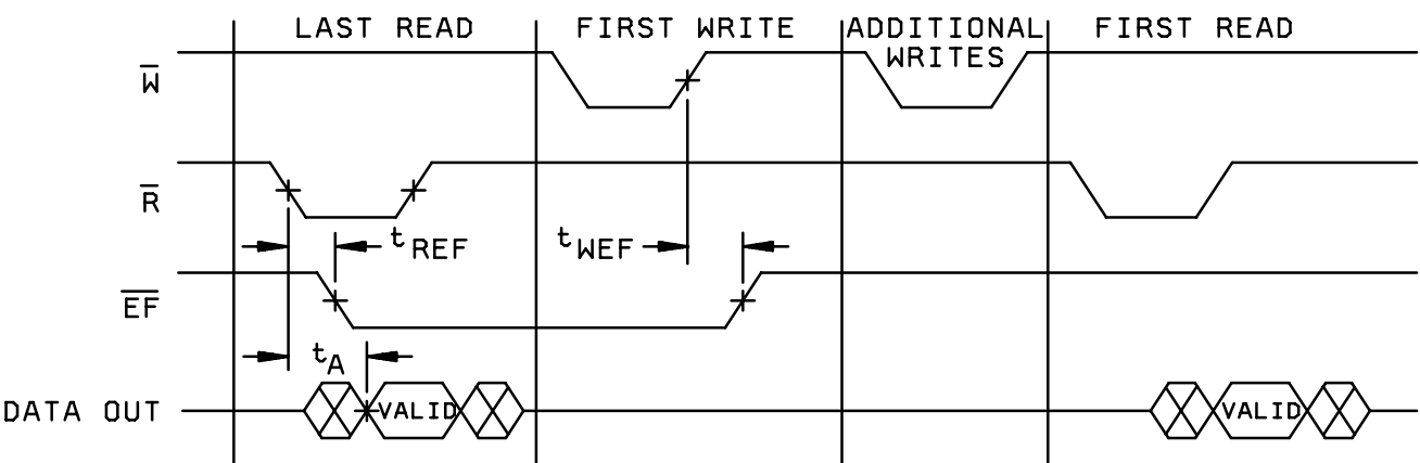
Last read to first write empty flag timing diagram
