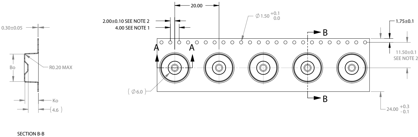
SECTION B-B
