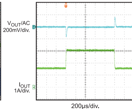
Load Transient I_{OUT} = 1.5A \leftrightarrow 3A , 1.6A/\mu s
