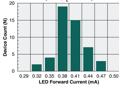
Typical LED Forward Current to Activate (N=50, I_L=100\text{mA} )
