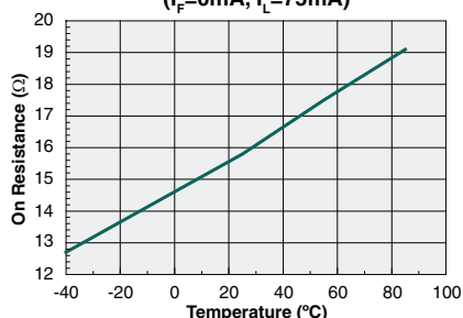
On-Resistance vs. Temperature ( I_F=0\text{mA} , I_L=75\text{mA} )
