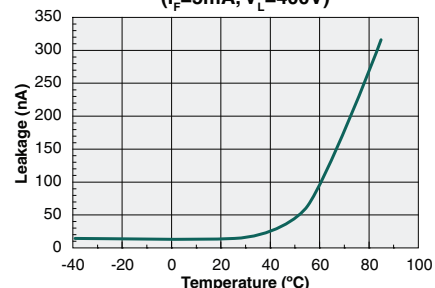
Typical Leakage vs. Temperature Measured Across Pins 5&6, 7&8 ( I_F=5\text{mA} , V_L=400\text{V} )
