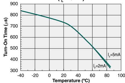
Turn-On Time vs. Temperature ( I_L=75\text{mA} )
