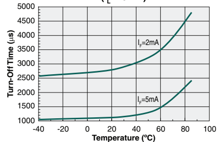
Turn-Off Time vs. Temperature ( I_L=75\text{mA} )
