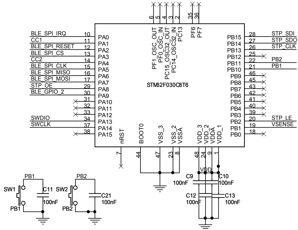
Figure 4. Microcontroller section
