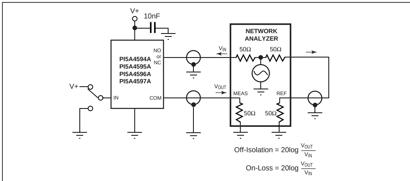
Figure 4. Off-Isolation and On-Channel Bandwidth
