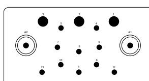
MOLDED 15C2
