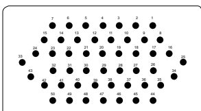
MOLDED 50
