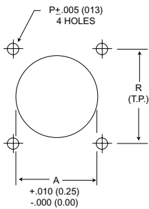
Box and Wall Mounting Receptacle
