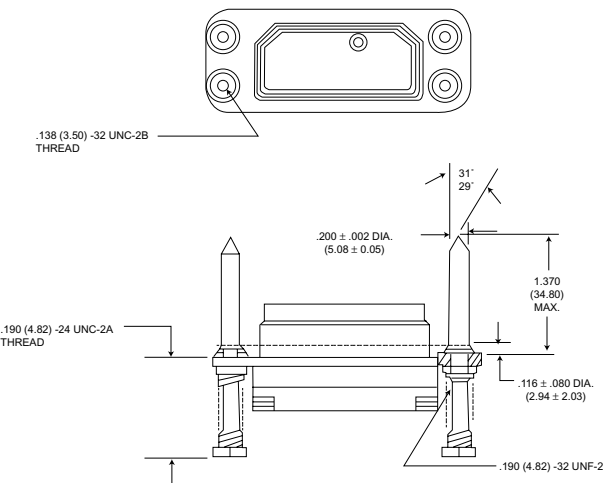
Mounting Style X - MIL-C-83733/2(USAF) With Guide Pins and Spring Mounting
