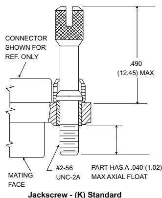
Jackscrew - (K) Standard
