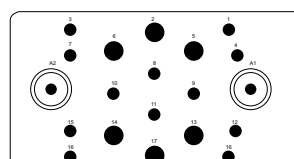
MOLDED B20C2
