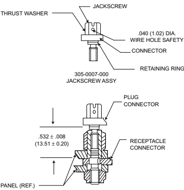
Mounting Spacing Dimensions For Jackscrew Assemblies
