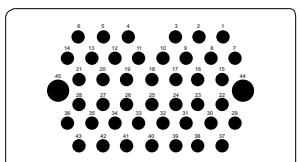
MOLDED 45
