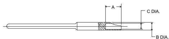
Pin/Solder Pot
