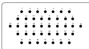
FABRICATED 40
