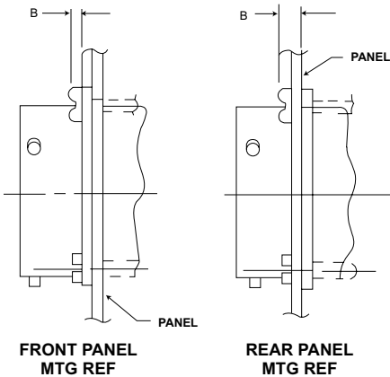
Wall Mounting and Box Mounting Receptacle
