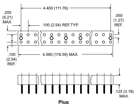
Plug
