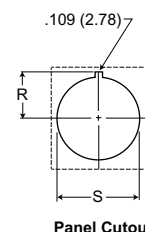
Panel Cutout
