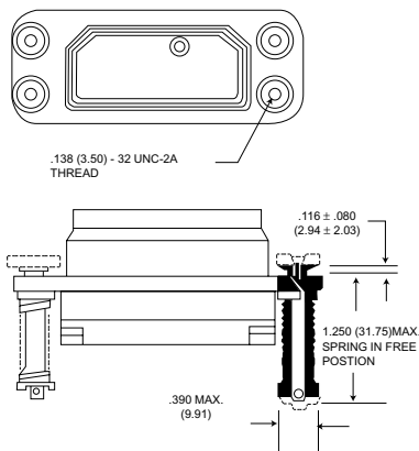
Mounting Style K - MIL-C-83733/4(USAF) With Captive Springs
