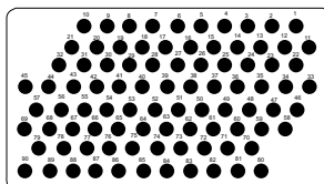
MOLDED 90
