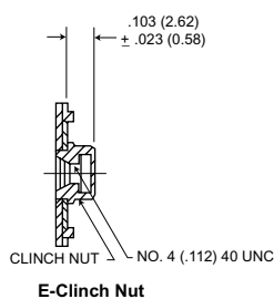
E-Clinch Nut
