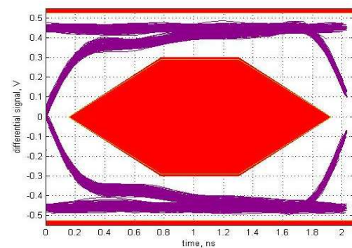
Figure 16. Downstream Port 3
