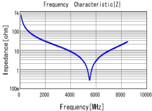
■ GCQ1555C1H2R5WB01 |Z| DC0V, 25degC
