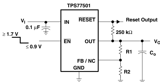
Figure 26. TPS77501 Adjustable LDO Regulator Programming
