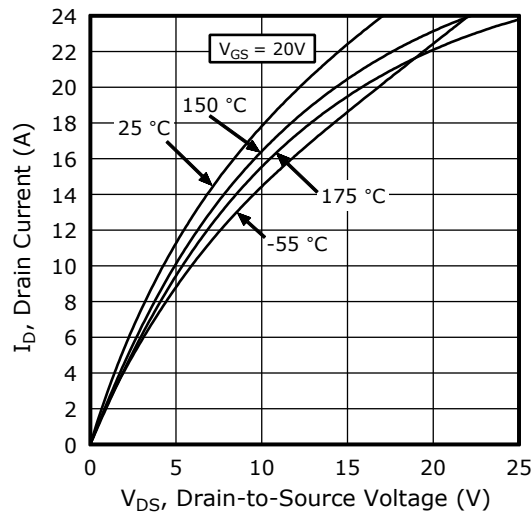
Figure 1-1. Drain Current vs. V_{DS} at T_J
