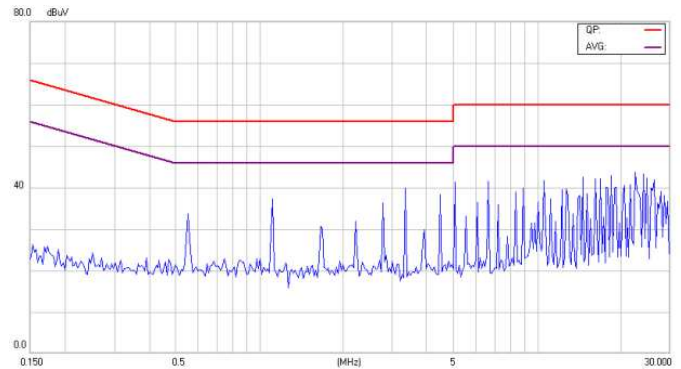
Conducted Class B of EC4SAW-24S33N
