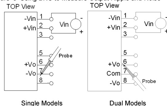
Figure 7 Using Probe to Measure Output Ripple and Noise
