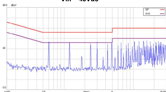
Conducted Class B of EC4SAW-48S05N Vin = 48Vdc
