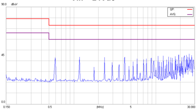
Conducted Class A of EC4SAW-24S12N
