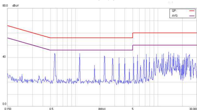
Conducted Class B of EC4SAW-48S15N Vin = 48Vdc
