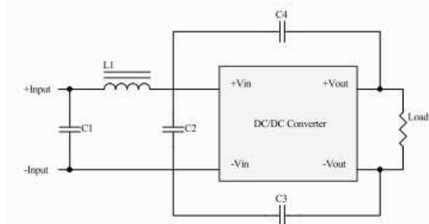
Figure 9 Connection circuit for conducted EMI testing
