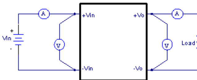
Figure 5 EC4SAW Series Test Setup
