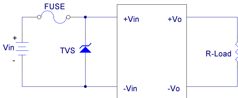
Figure 8 Input Protection
