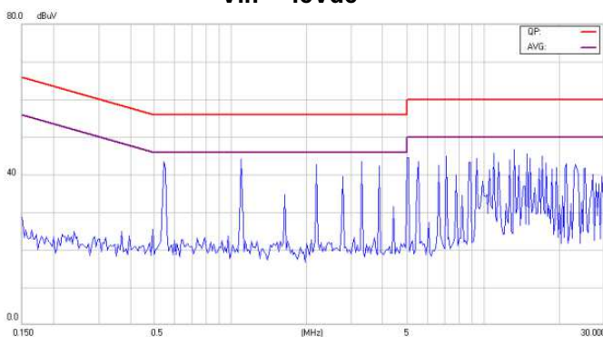
Conducted Class B of EC4SAW-48S12N Vin = 48Vdc
