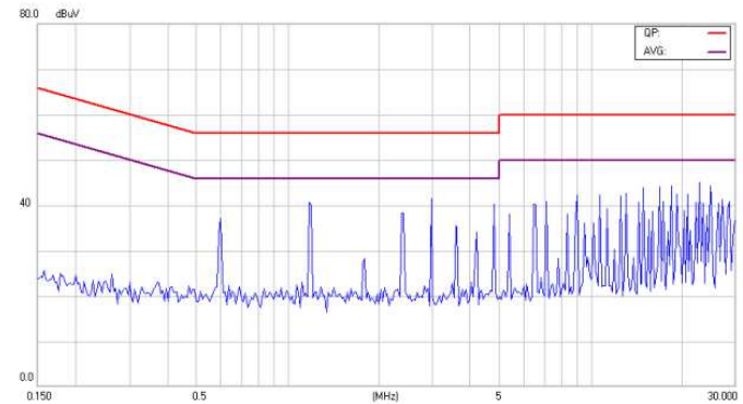
Conducted Class B of EC4SAW-24S05N
