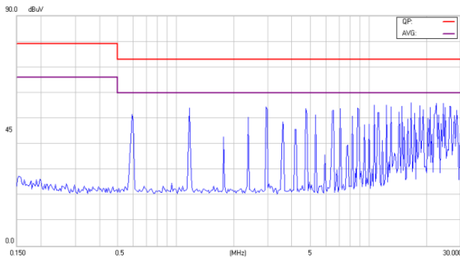
Conducted Class A of EC4SAW-24D05N Vin = 24Vdc
