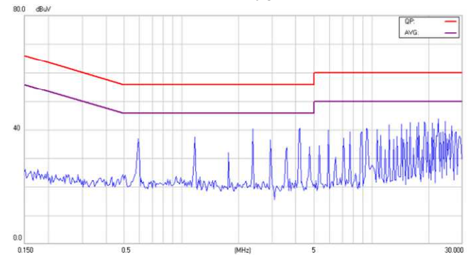
Conducted Class B of EC4SAW-24S12N
