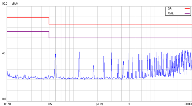
Conducted Class A of EC4SAW-24S05N
