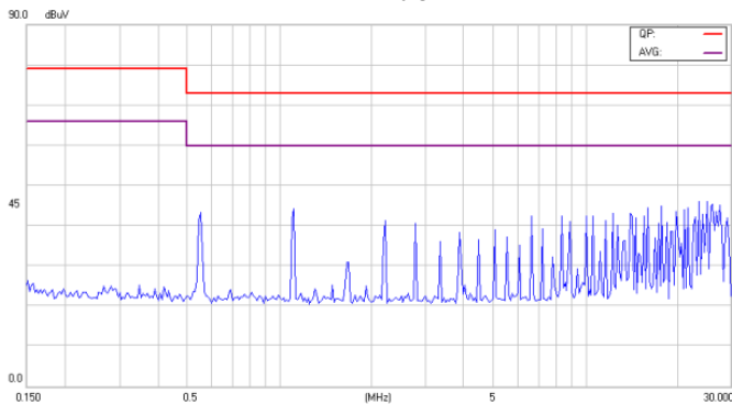
Conducted Class A of EC4SAW-24S33N
