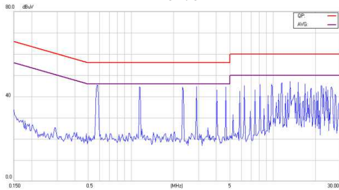
Conducted Class B of EC4SAW-48D05N
