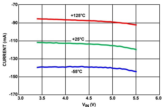
FIGURE 120. SHORT-CIRCUIT TO GND
