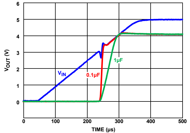
FIGURE 131. TURN-ON TIME
