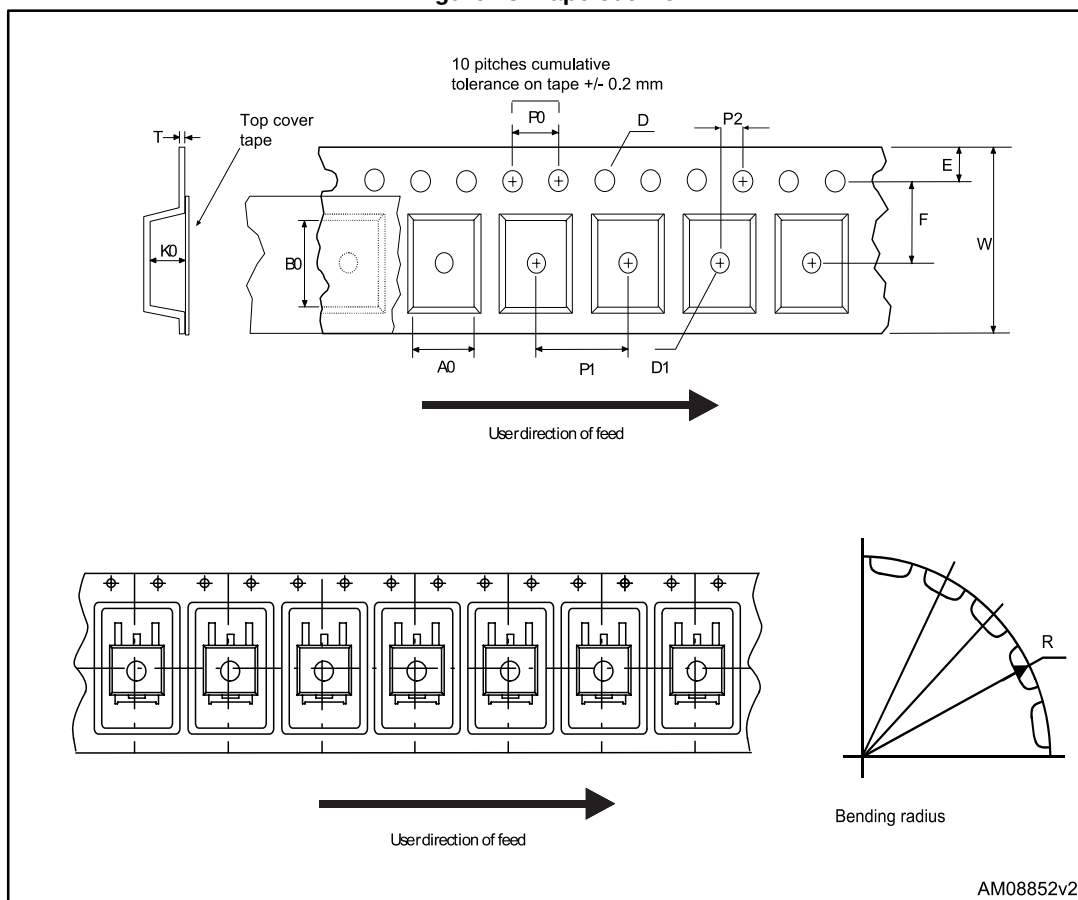
Figure 23: Tape outline
