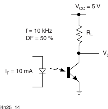
Fig. 14 - Switching Schematic
