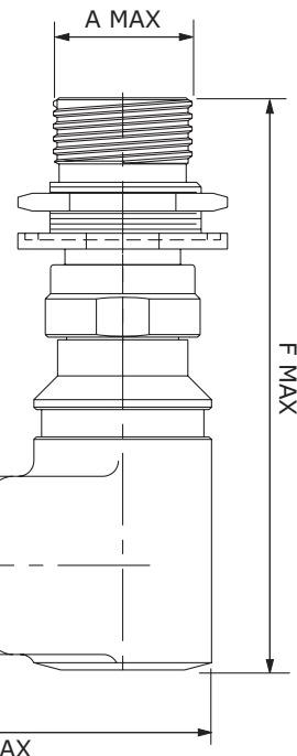
M28876/14 Jam Nut Receptacle with 90° Backshell
