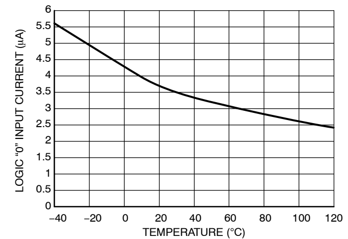
Figure 28. Logic "0" Input Current vs. Temperature
