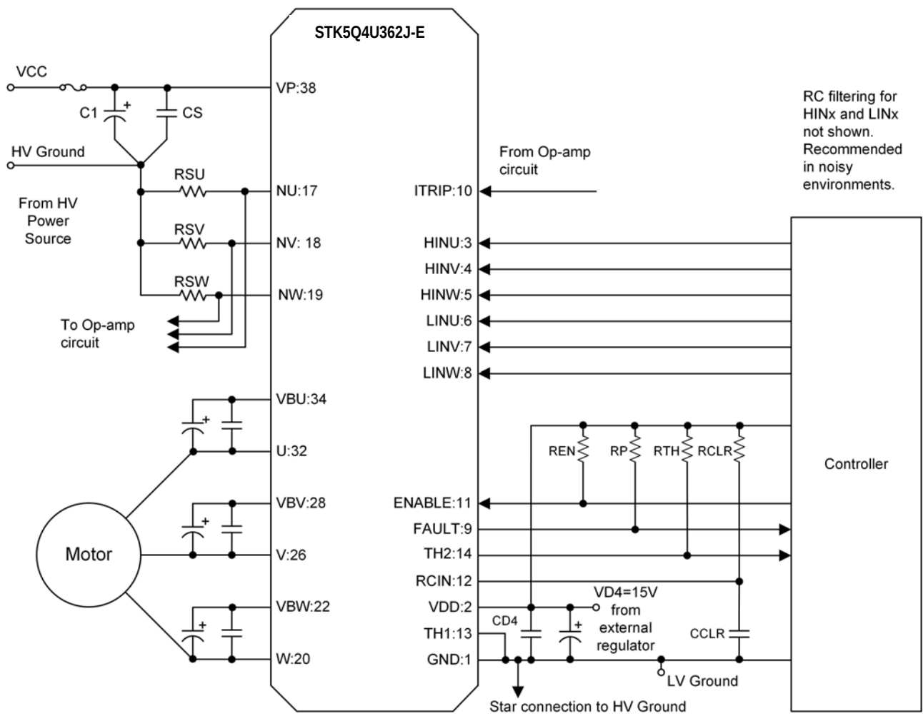
Figure 2. Application Schematic
