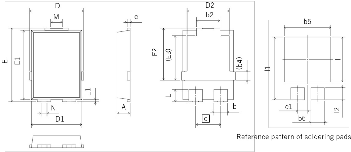
TO-277A, (TO-277GE)
