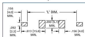
Pad Layout
