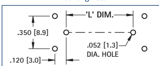
Mounting Detail
