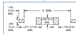
Pad Layout
