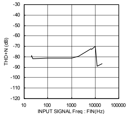
Fig.7 16bit D/A Converter Total Harmonic Distortion (Rch)
