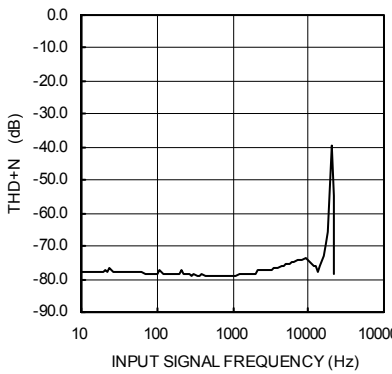
Fig.20 16bit D/A Converter Total Harmonic Distortion (SPOL)
