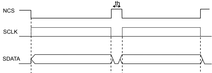
Fig.33 CPU I/F Timing Chart 2 (BU7858KN)
