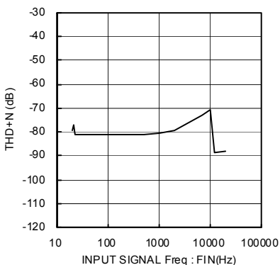
Fig.6 16bit D/A Converter Total Harmonic Distortion (Lch)
