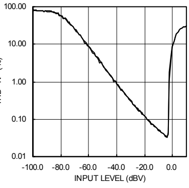
Fig.22 Headphone Amplifier Total Harmonic Distortion (HPOL / HPOR)
