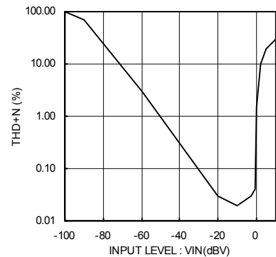
Fig.10 SPO Total Harmonic Distortion
