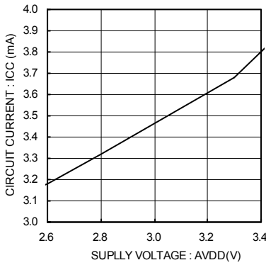
Fig.17 AVDD Operation Current (digital melody)
