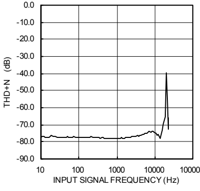
Fig.21 16bit D/A Converter Total Harmonic Distortion (SPOR)
