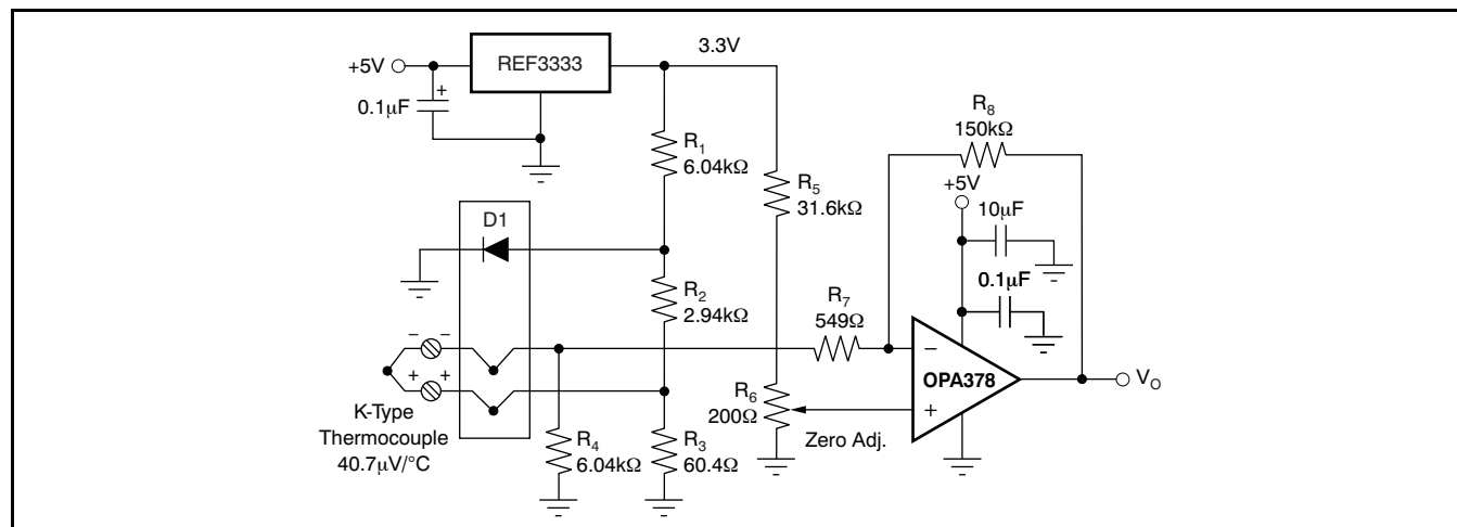
Figure 34. Temperature Measurement
