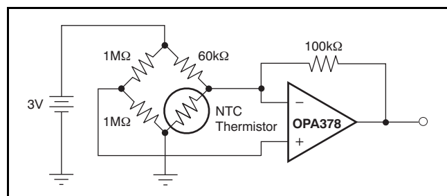
Figure 35. Thermistor Measurement
