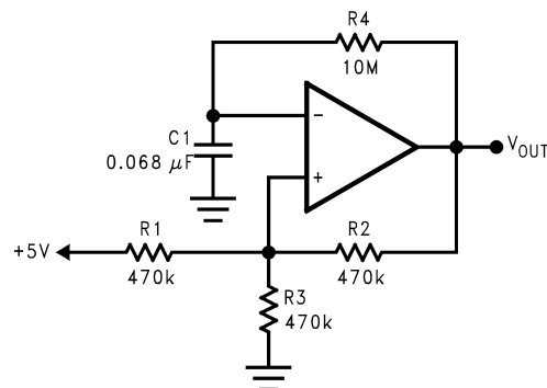
Figure 46. 1 Hz Square-Wave Oscillator
