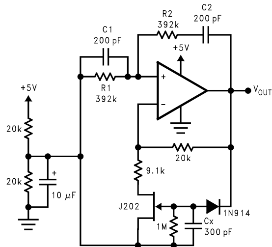
Figure 45. Sine-Wave Oscillator
