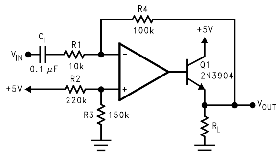
Figure 47. Power Amplifier
