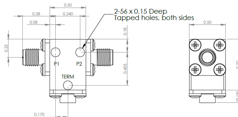
D3I3841 Dimensions
