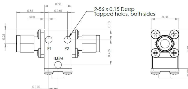
D3I3841-3 Dimensions
