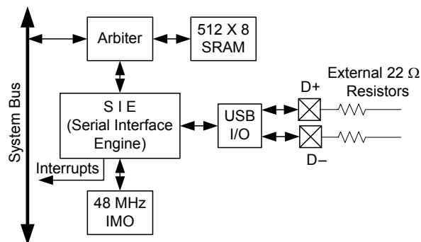
Figure 7-20. USB
