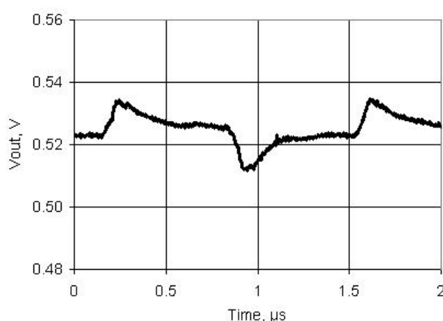
Figure 11-65. VDAC Voltage Noise, 1 V Mode, High speed mode, Vdda = 5 V
