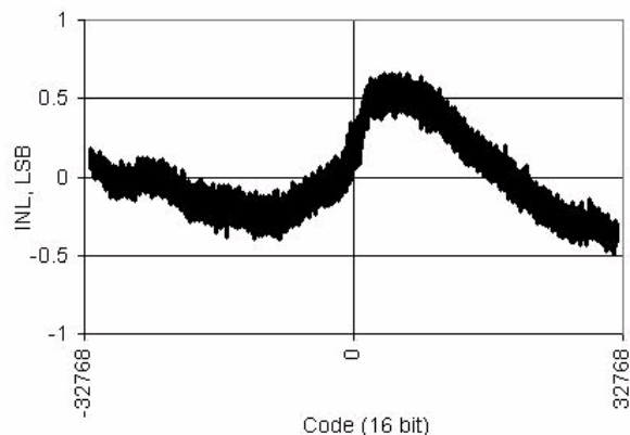
Figure 11-37. Delta-sigma ADC INL vs Output Code, 16-bit, 48 ksp/s, 25 °C V_{DDA} = 3.3 V
