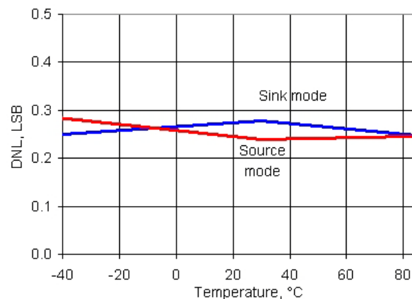
Figure 11-45. IDAC DNL vs Temperature, Range = 255 \mu A, High speed mode
