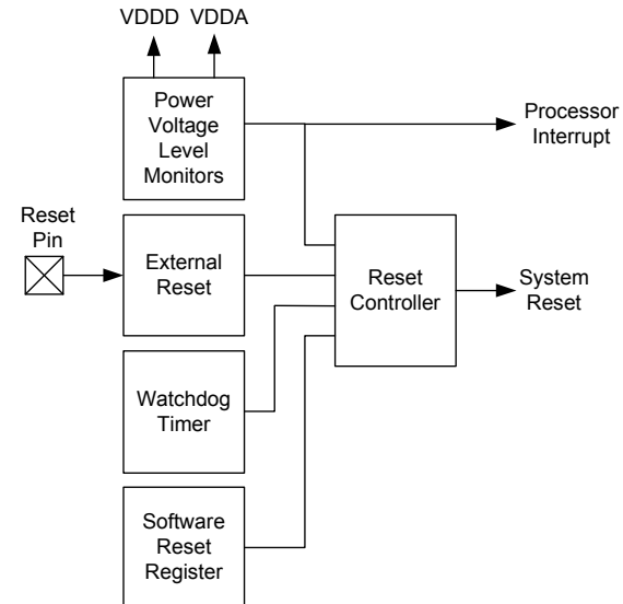
Figure 6-7. Resets
