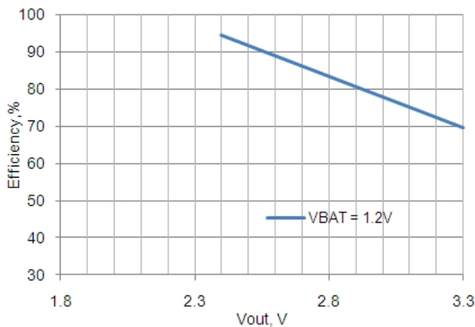
Figure 11-10. Efficiency vs V_{\text{OUT}} I_{\text{OUT}} = 75 \text{ mA} , V_{\text{BAT}} = 1.2 \text{ V}
