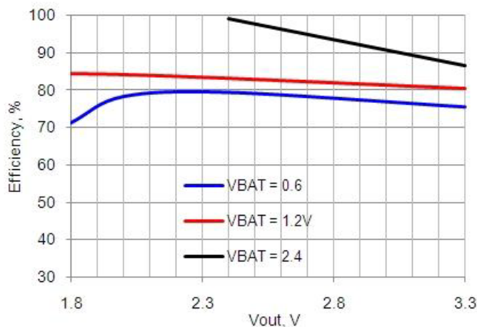
Figure 11-8. Efficiency vs V_{\text{OUT}} I_{\text{OUT}} = 5 \text{ mA} , V_{\text{BAT}} = 0.6 \text{ V} , 1.2 \text{ V} , and 2.4 \text{ V}
