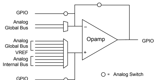
Figure 8-7. Opamp
