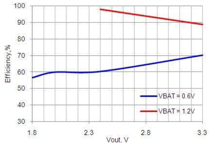
Figure 11-9. Efficiency vs V_{\text{OUT}} I_{\text{OUT}} = 30 \text{ mA} , V_{\text{BAT}} = 0.6 \text{ V} and 1.2 \text{ V}
