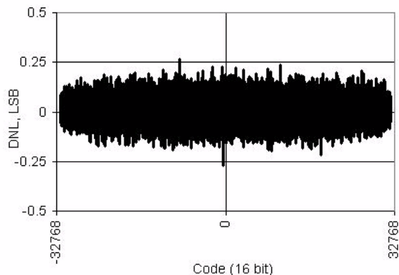
Figure 11-36. Delta-sigma ADC DNL vs Output Code, 16-bit, 48 ksp/s, 25 °C V_{DDA} = 3.3 V
