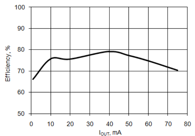
Figure 11-11. Efficiency vs I_{\text{OUT}} V_{\text{BAT}} = 2.4 \text{ V} , V_{\text{OUT}} = 3.3 \text{ V}
