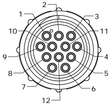
WIRE VIEW
