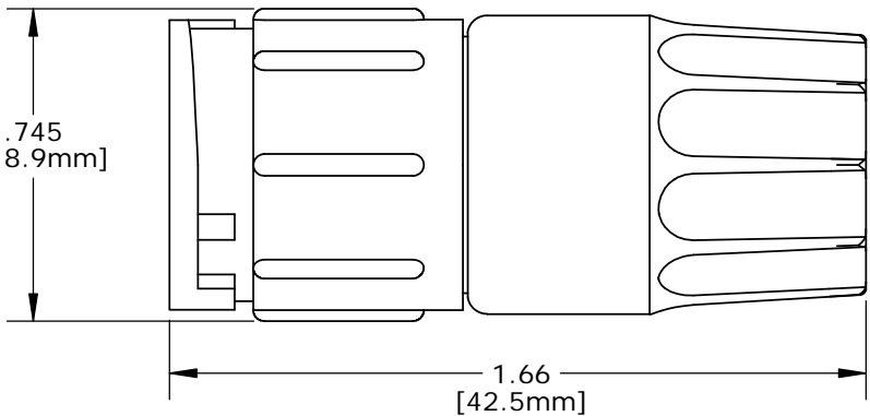
ASSEMBLED VIEW
