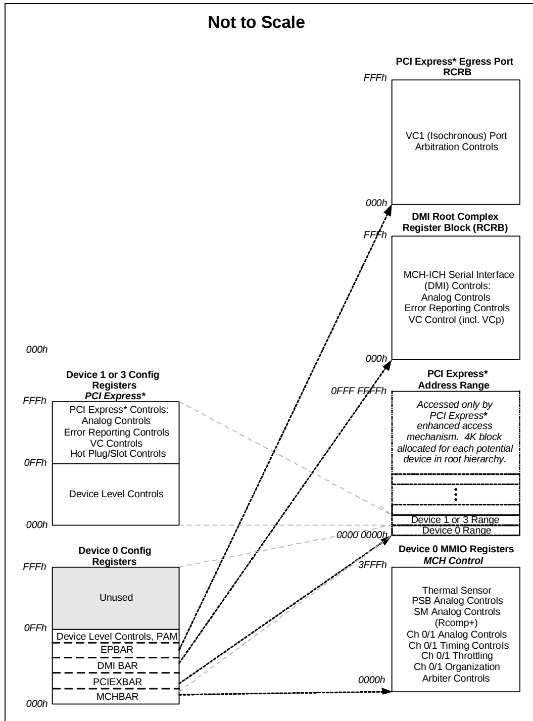
Figure 3-2. Register Organization
