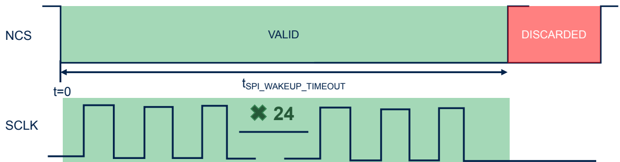
Figure 5. Wake-up condition by peripheral SPI
