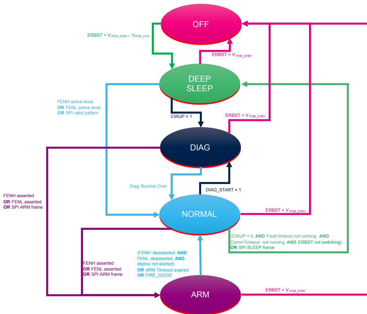
Figure 3. Device FSM
