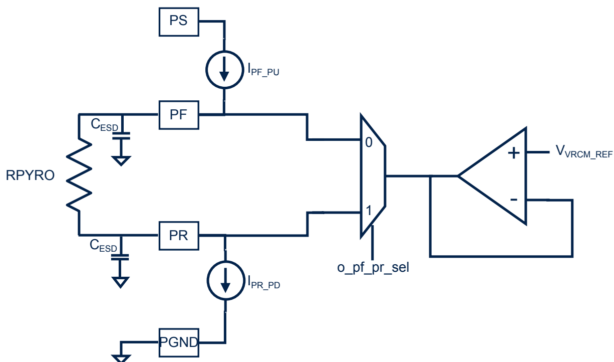
Figure 20. VRCM test
