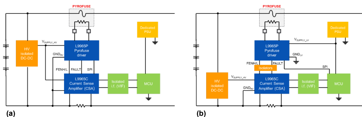
Figure 34. Pyro-fuse driver positioning
