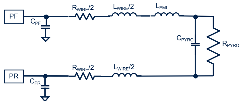
Figure 16. Pyro-fuse input model
