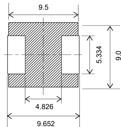
PCC-M1040M-LP type (ETQP4M1R0KVC)
