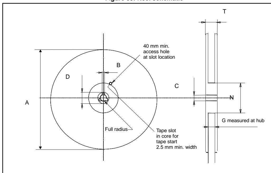
Figure 33: Reel schematic
