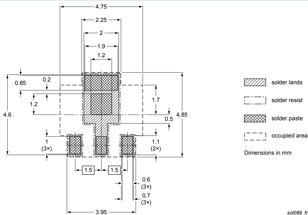
Fig. 13. Reflow soldering footprint for SOT89
