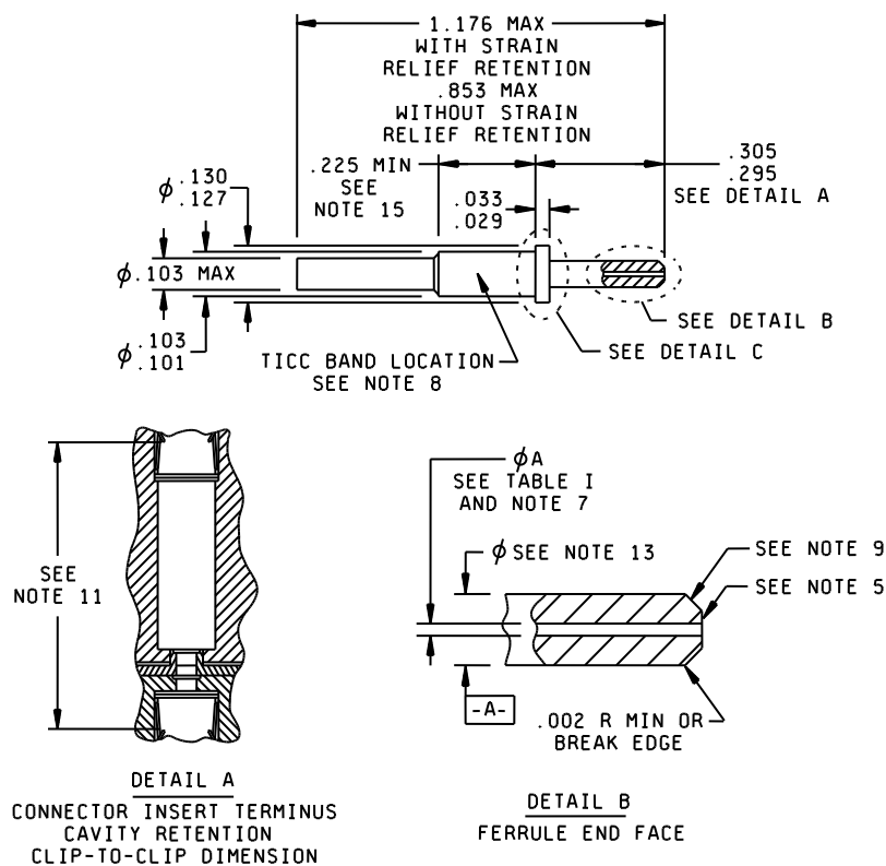
FIGURE 1. Pin terminus
