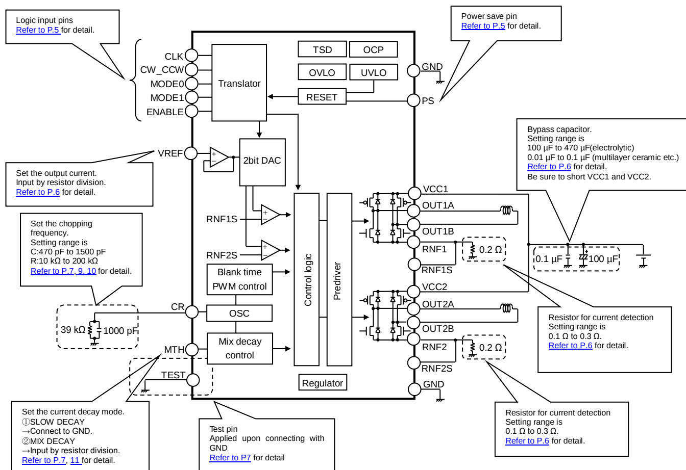
Figure 8. BD63716AMWV Block Diagram and Applied Circuit Diagram
