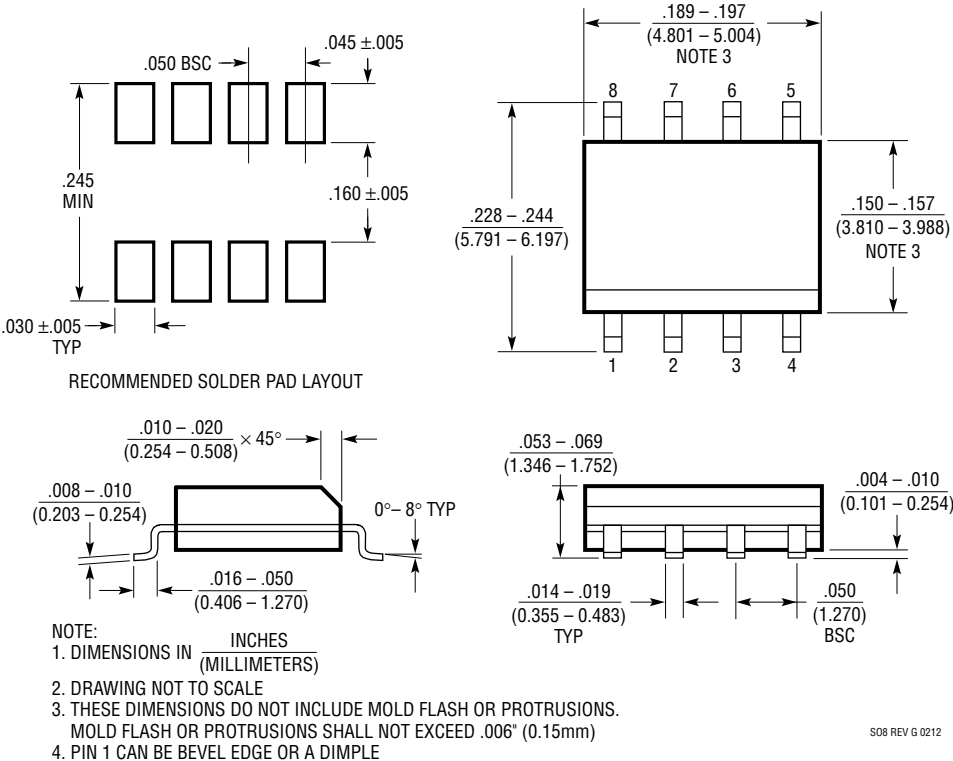
S8 Package 8-Lead Plastic Small Outline (Narrow .150 Inch) (Reference LTC DWG # 05-08-1610 Rev G)
