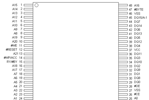
Figure 3-3-4 48-PIN STANDARD TSOP (TOP VIEW)
