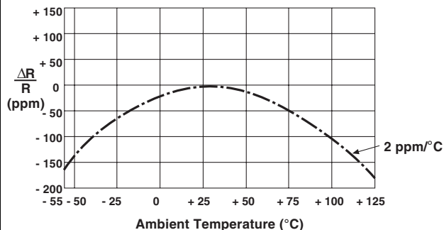
FIGURE 4 - TYPICAL RESISTANCE/ TEMPERATURE CURVE
