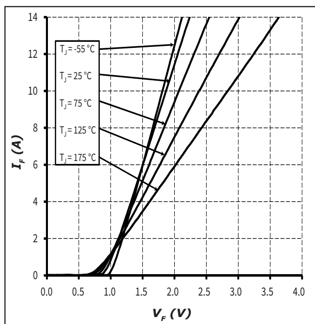
Figure 1. Forward Characteristics
