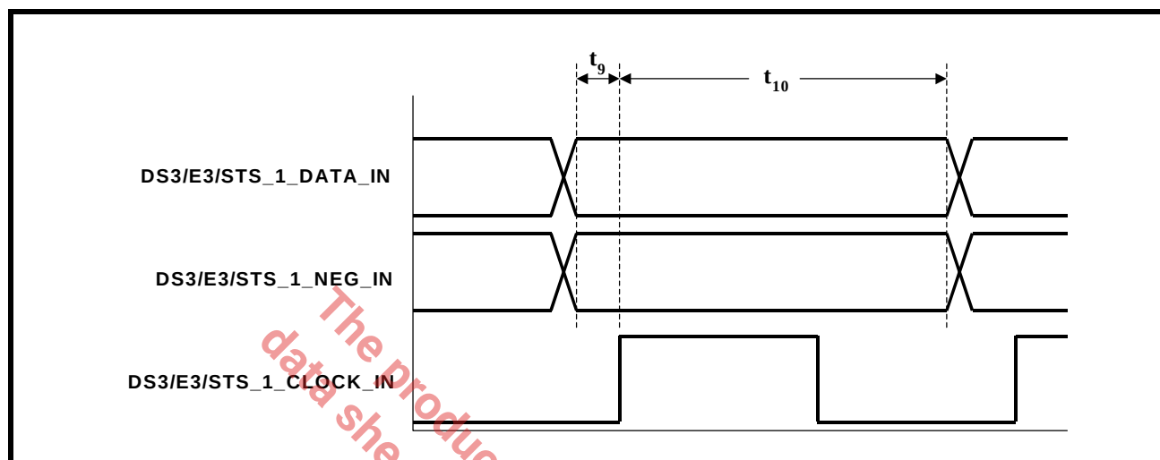
FIGURE 18. WAVEFORMS OF THE DS3/E3/STS-1 SIGNALS THAT ARE INPUT TO THE DS3/E3/STS-1 LIU INTERFACE IN THE INGRESS DIRECTION
