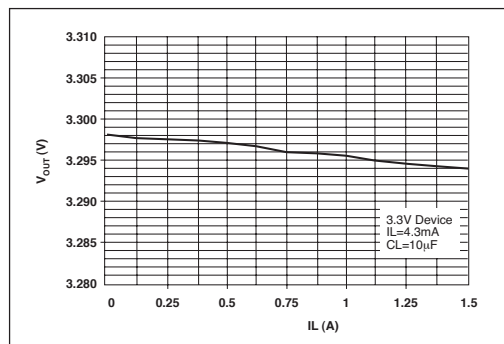
Figure 3. Load Regulation
