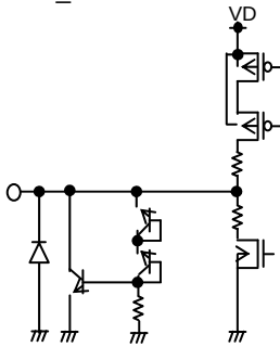
2pin&lt;SS_V3&gt;
