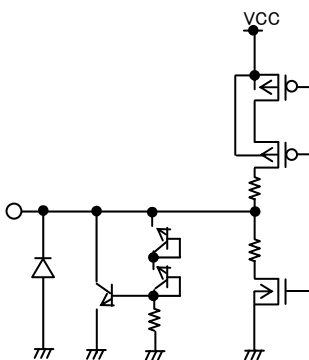
16pin&lt;SS_V15&gt;
