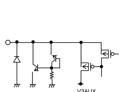
20pin&lt;V3AUX_IN&gt;
