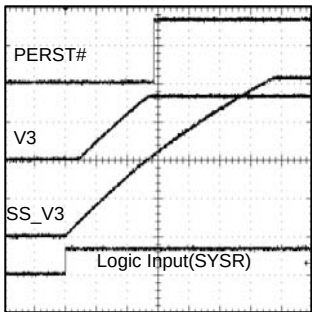
Fig.9 V3 Start up (Stand-by→Active)
