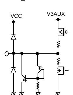
6pin&lt;SS_V3AUX&gt;
