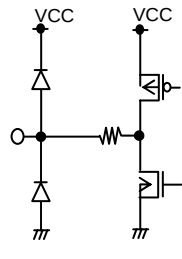
13pin&lt;PERST#_DELAY&gt;
