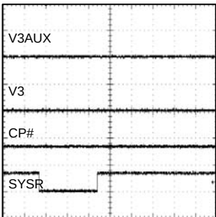
Fig. System Stand-by⇄Active (No Card)
