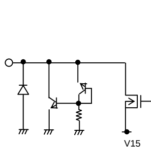
17,18pin&lt;V15_IN1,V15_IN2&gt;
