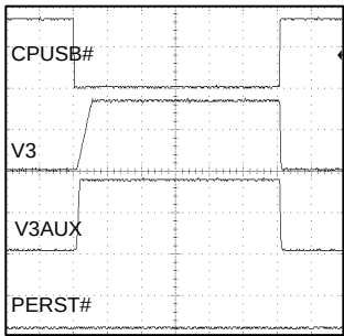
Fig.6 USB Card Assert/ DeAssert (Active)
