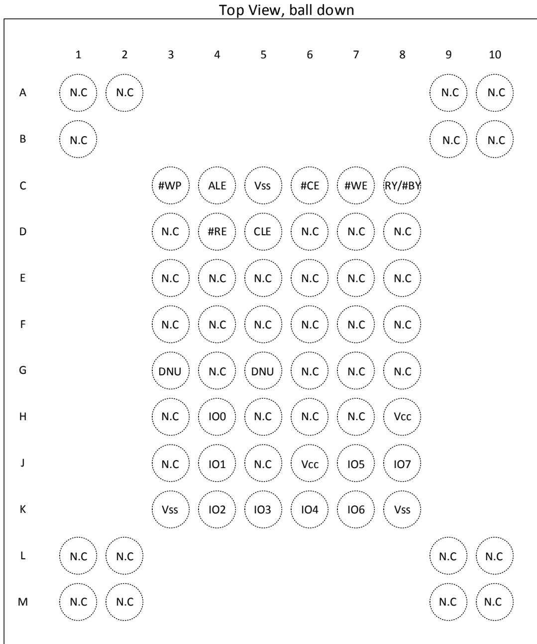
Figure 3-2 Pin Assignment 63-ball VFBGA (Package code B)
