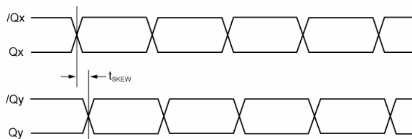
Figure 1c. Output-to-Output Skew
